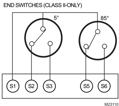
Fig. 9. End Switches.
